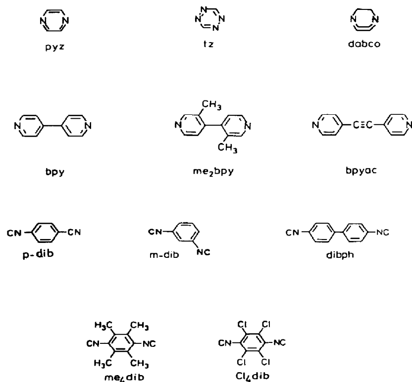
Fig. 3. Bridging ligands pyrazine (pyz), 1,2,4,5-tetrazine (tz), diazabicyclo[2.2.2]octane (dabco), 4,4'-bipyridine (bpy), 2,2'-dimethyl-4,4'-bipyridine (me 2 bpy), bipyridylacetylene (bpyac), p -diisocyanobenzene (dib), m -diisocyanobenzene ( m -dib), diisocyanobiphenyl (dibph), tetramethyldiisocyanobenzene (me 4 dib) and tetrachlorodiisocyanobenzene (Cl 4 dib).
