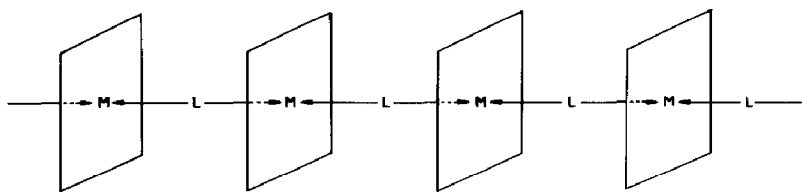
Fig. 1. Bridged macrocyclic transition metal polymers: \boxed{M} = metallomacrocycle; L = bidentate bridging ligand.
